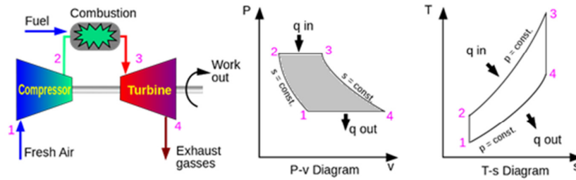
Figure 2: Representation of the ideal Brayton Cycle
