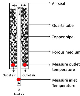
Figure 3: Representation of the air flow through the system
