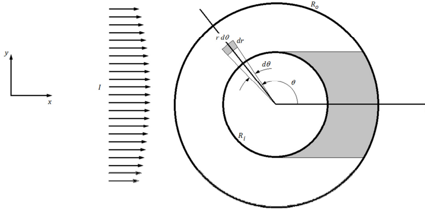
Figure 4: Attenuation of a radiation beam passing through porous medium.
