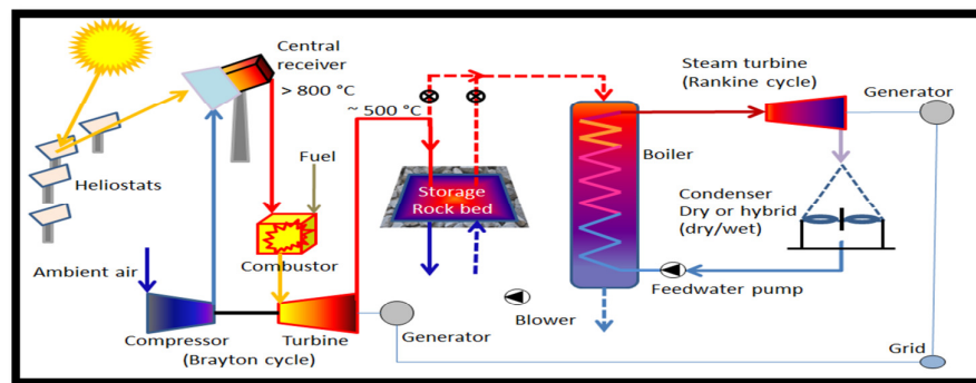
Figure 1: Representation of Basic SUNSPOT cycle [1]
