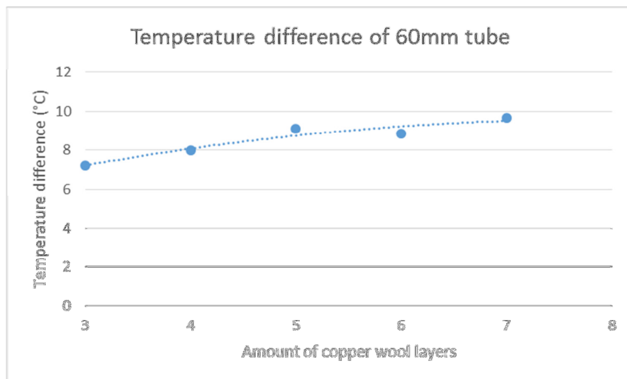
Figure 5: Increase in temperature with regards to the volume porous medium
