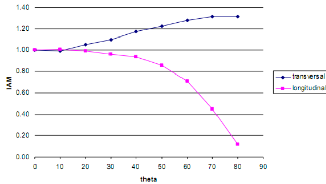
Fig. 3: Dependence of IAM of incidence angle theta of the sun beams (Häberle et al., 2002)
