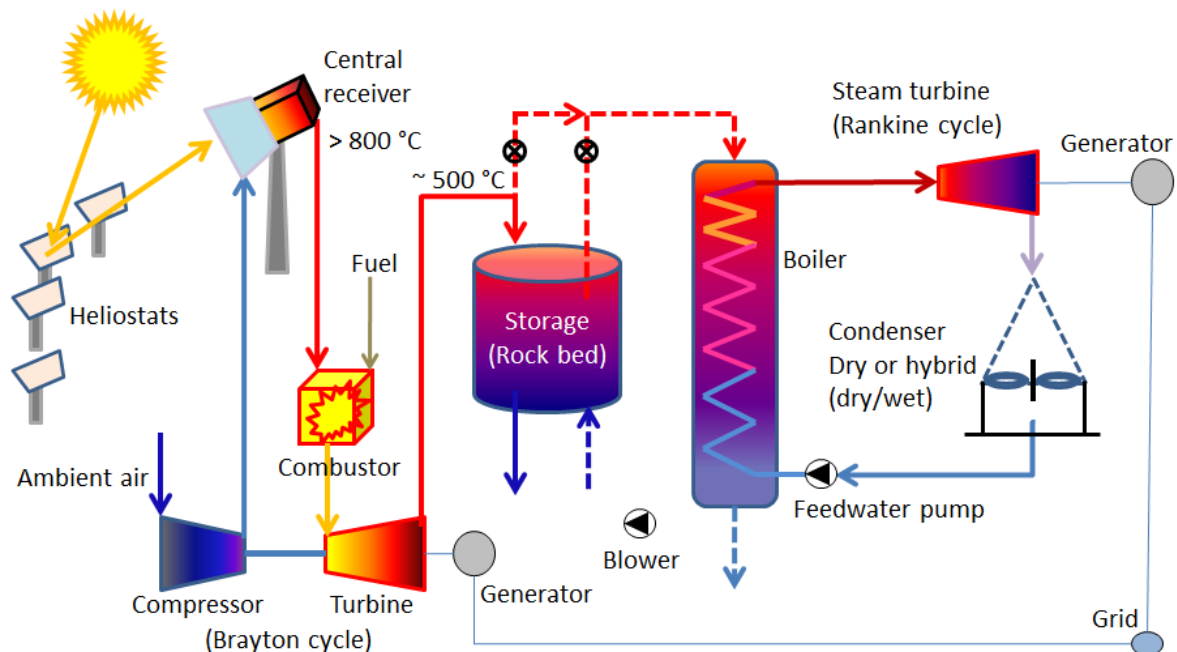
Figure 1: The SUNSPOT cycle (courtesy of K. Allen).
