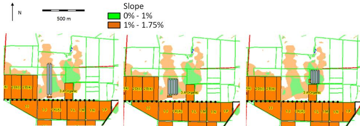
Fig. 6: Possible linear Fresnel plant setup with two lines (left) and four lines (middle and right)
